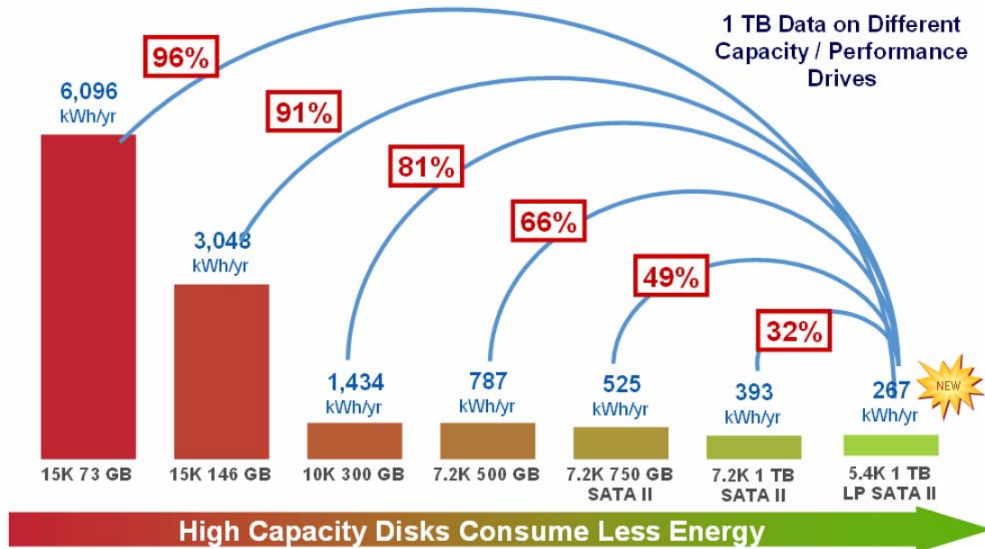
Figure 3 Power consumption of various drive types
